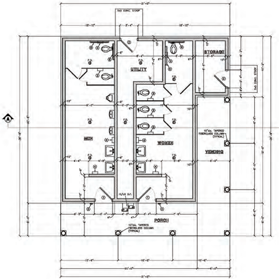
Floor Plan
