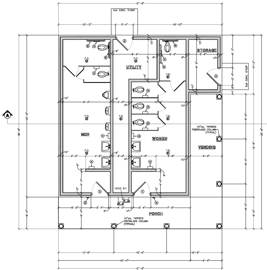
Floor Plan
